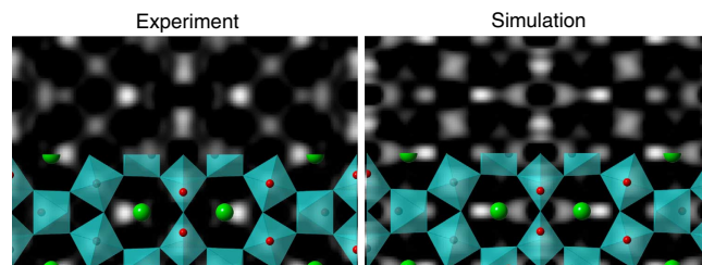
Figure 2 | Comparison of bulk-subtracted experimental and simulated HRTEM images. Experimental (left) and simulated (right) HRTEM images of the SrTiO 3 (001) c(6 \times 2) Sr7 surface reconstruction on a 5.3-nm-thick sample at a defocus of 0.55 nm with bulk subtraction and corrected for the top/bottom surface registry shift with phases inverted 180 degrees for spatial frequencies where \sin(\chi) < 0 in the phase contrast transfer function.
