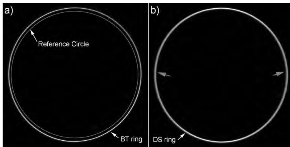
Figure E.2. Reciprocal space alignment on the JEOL 3000F systems described in appendix C. (a) shows the BT ring alignment and (b) shows the complementary descan alignment. The x and y descan coils do not have the same number of windings on this instrument. Consequently, the precision of the DACs is more limited in one axis, leading to a slight broadening of the ring indicated by the grey arrows.
